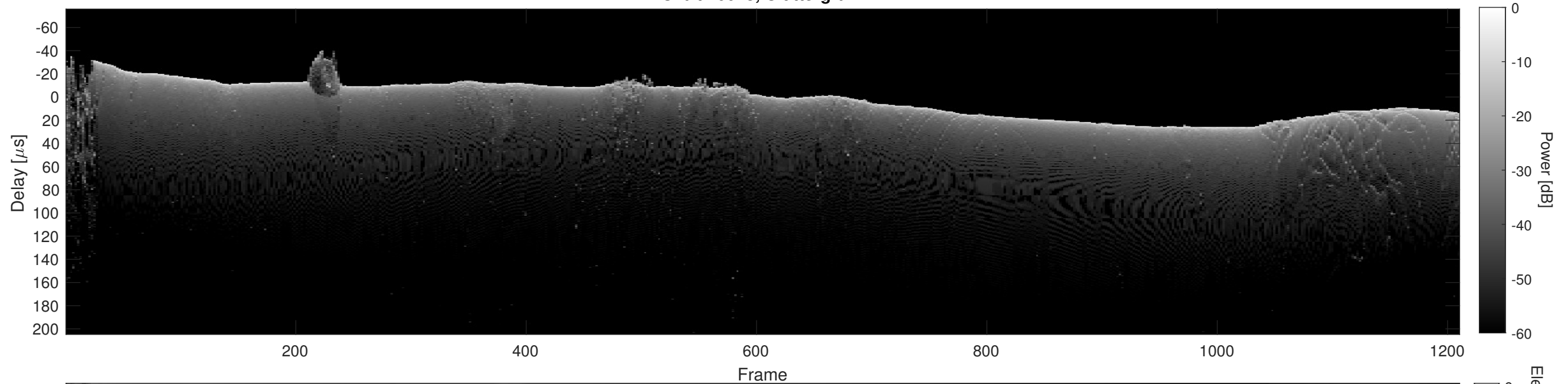
Orbit 10043, Cluttergram
