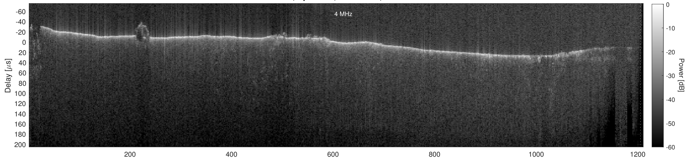
Orbit 10043, Cluttergram
