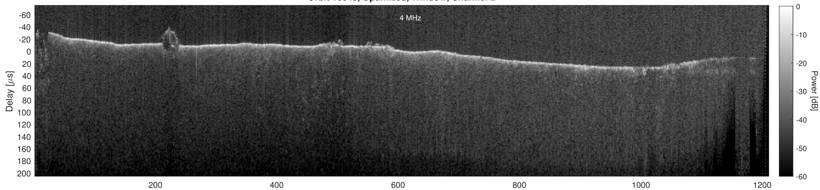
Orbit 10043, Cluttergram
