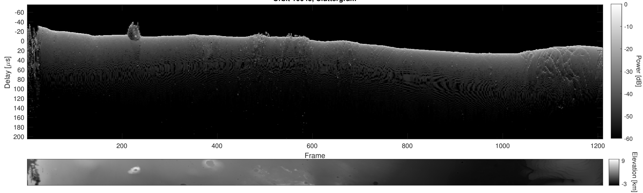
Orbit 10043, Cluttergram
