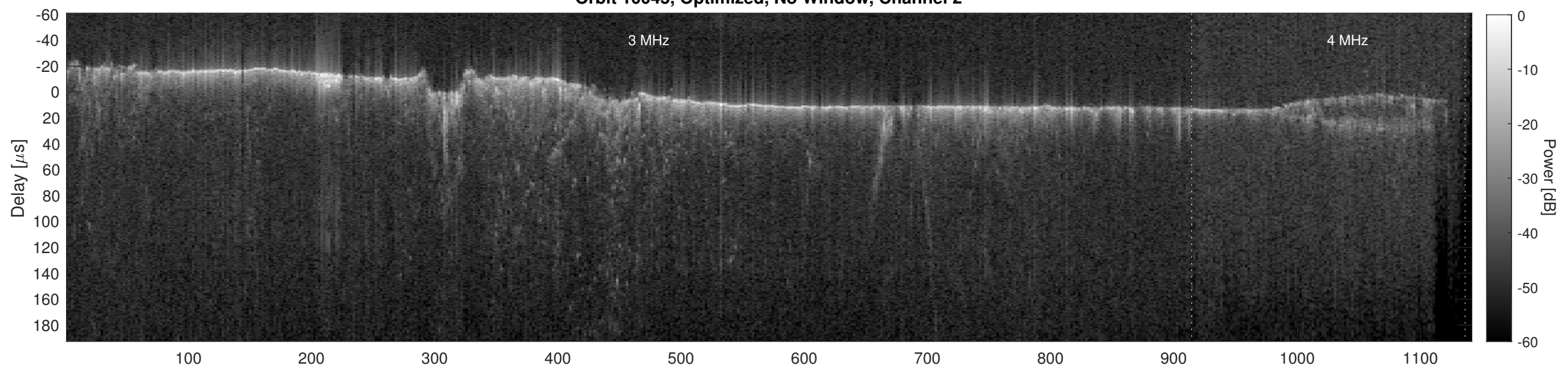
Orbit 10045, Cluttergram
