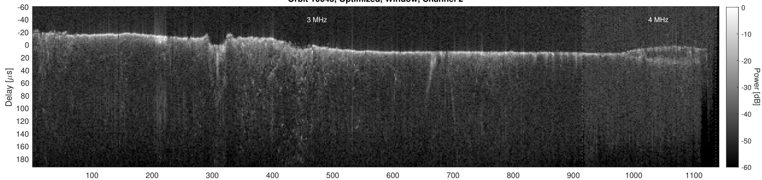
Orbit 10045, Cluttergram
