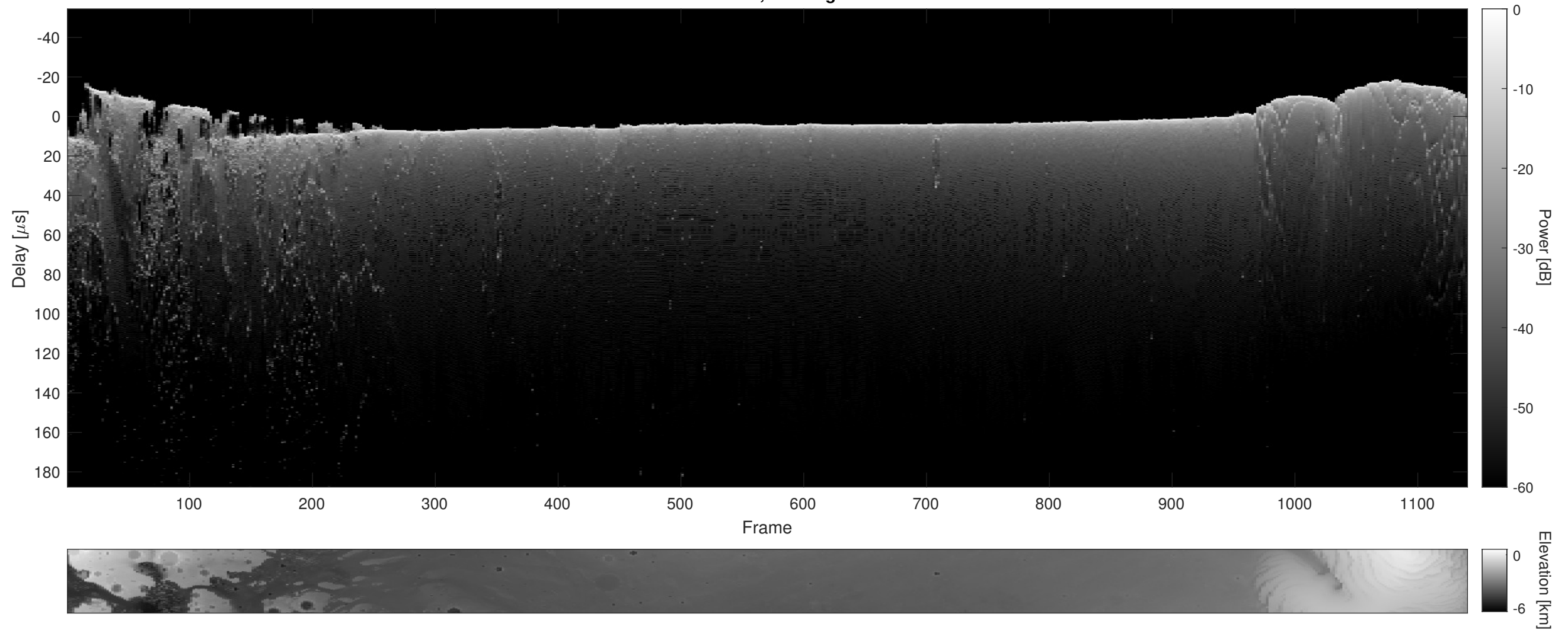
Orbit 10046, Cluttergram
