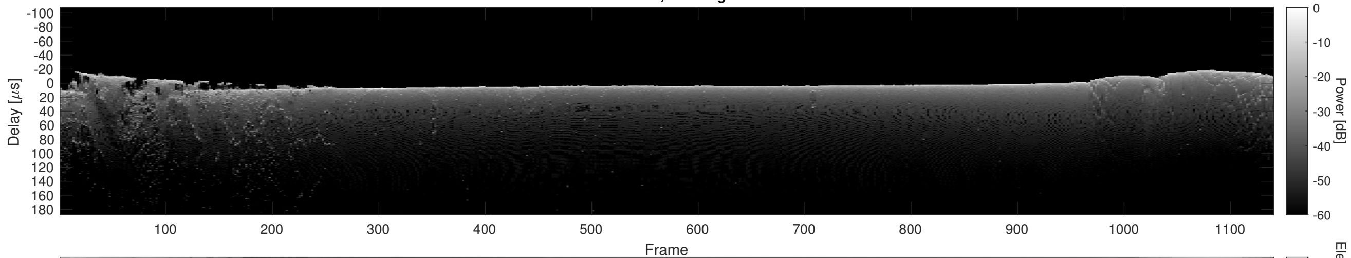
Orbit 10046, Cluttergram
