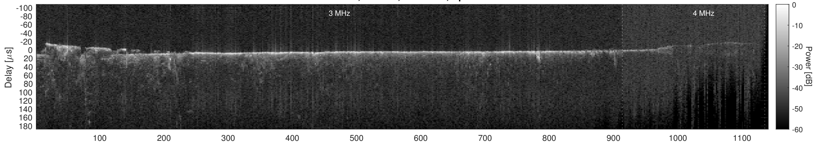
Orbit 10046, Cluttergram
