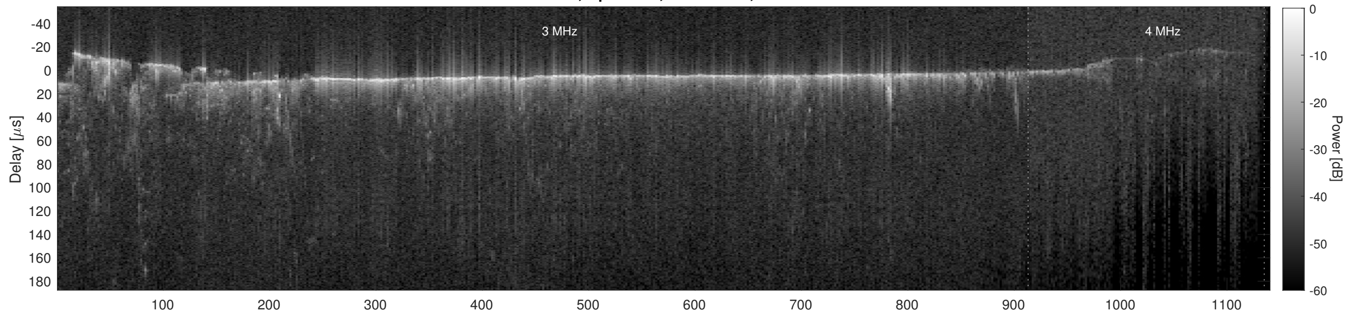
Orbit 10046, Cluttergram
