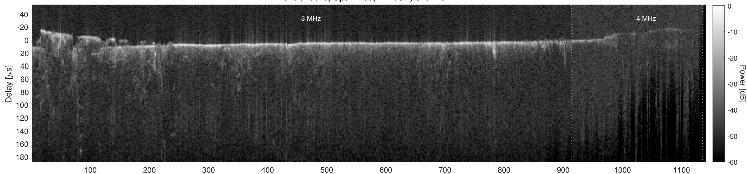
Orbit 10046, Cluttergram
