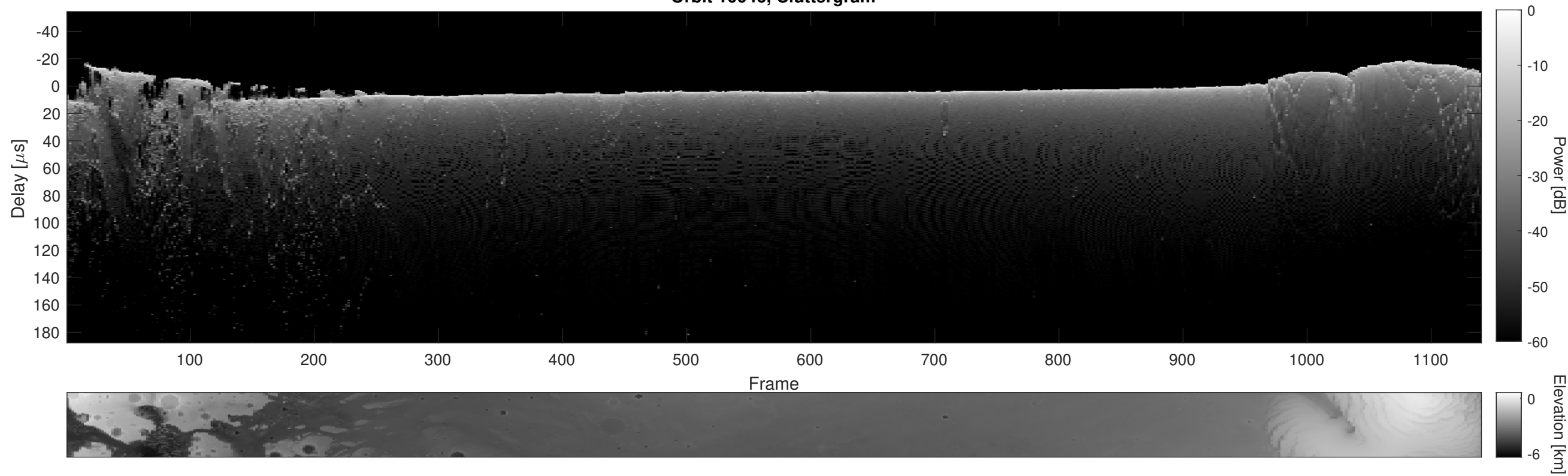
Orbit 10046, Cluttergram
