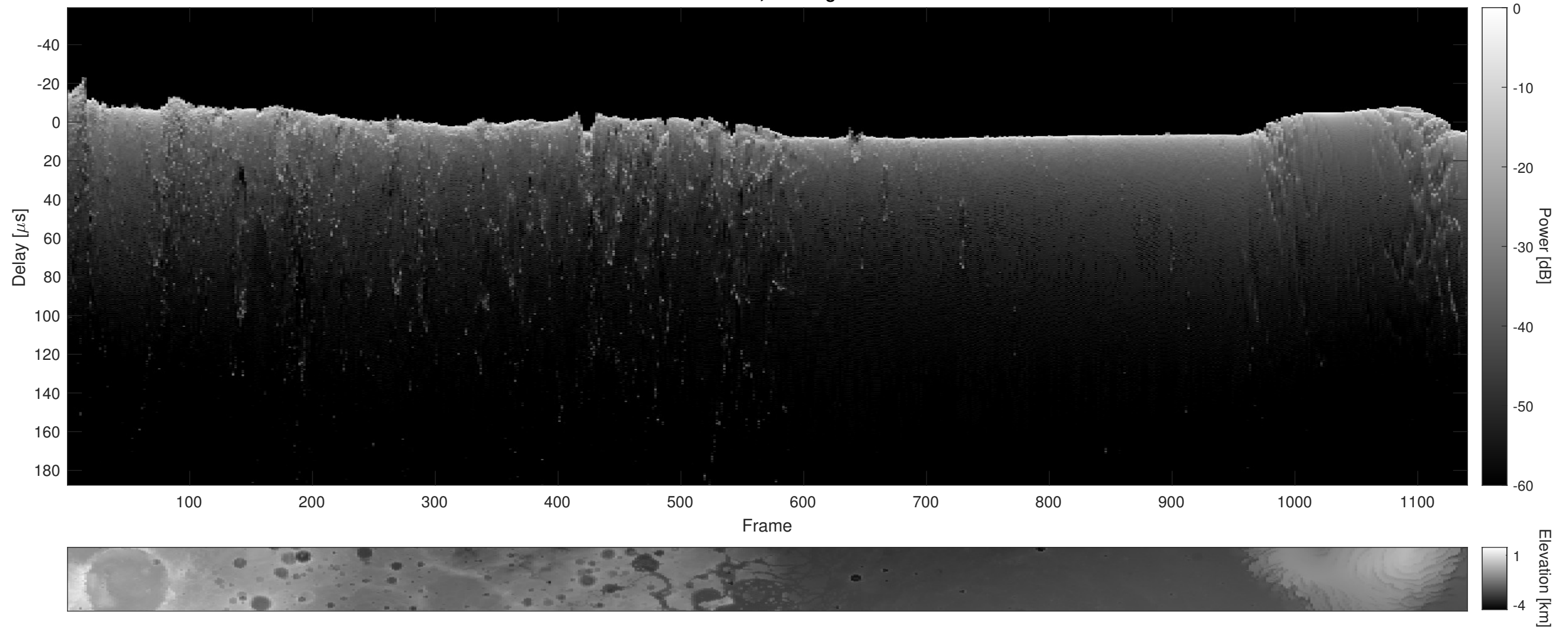
Orbit 10049, Cluttergram
