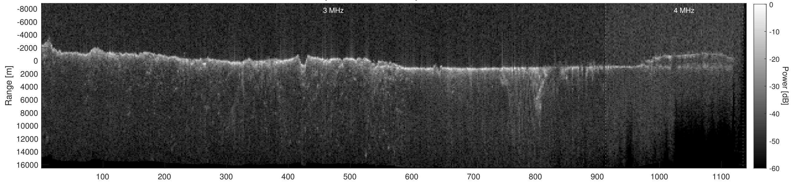
Orbit 10049, Depth-Corrected Cluttergram
