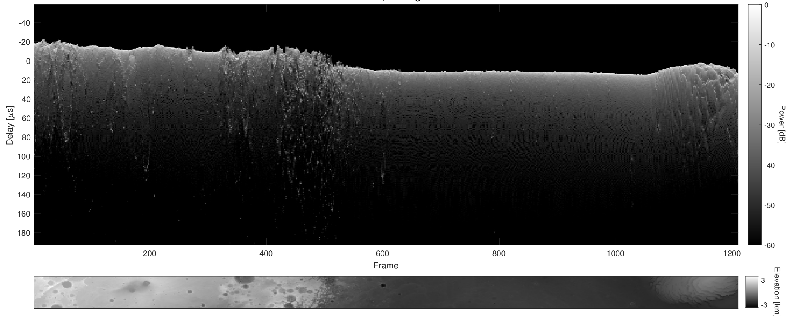
Orbit 10052, Cluttergram
