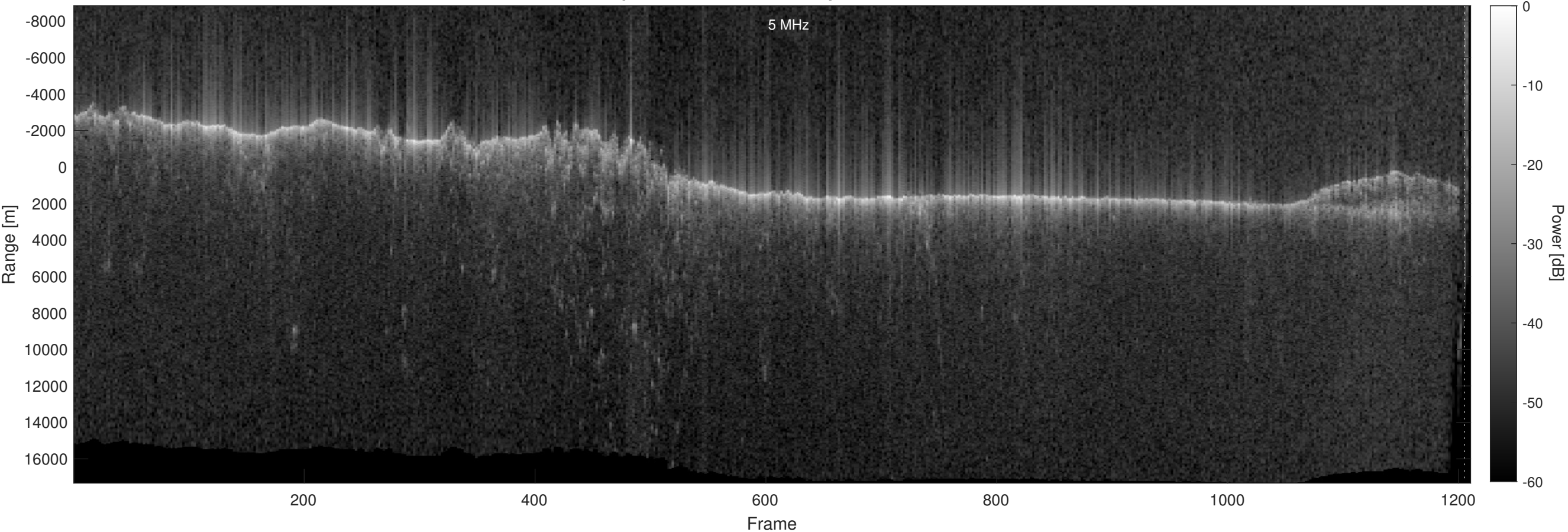
Orbit 10052, Optimized, No Window, Depth-Corrected, Channel 2
