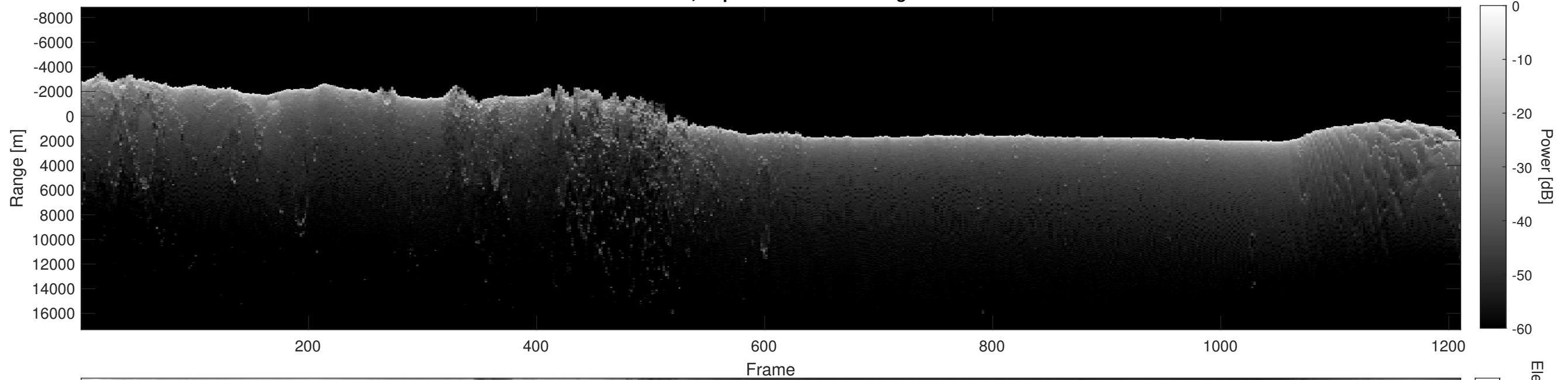
Orbit 10052, Depth-Corrected Cluttergram
