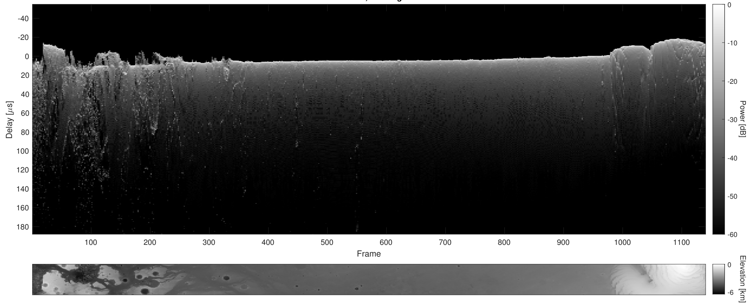
Orbit 10053, Cluttergram
