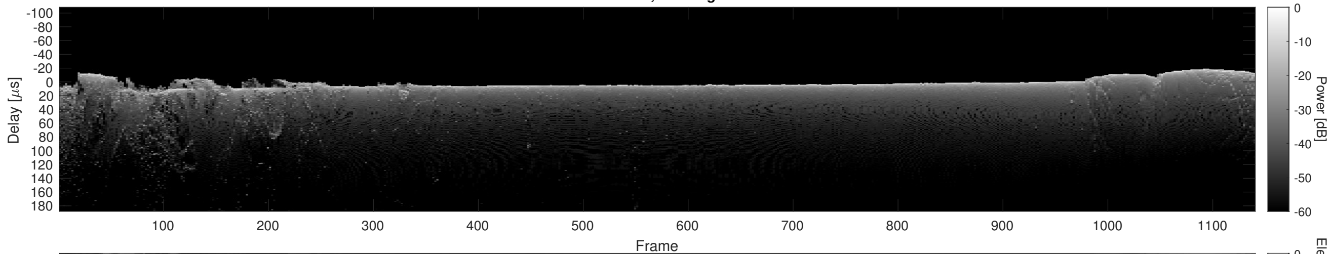
Orbit 10053, Cluttergram
