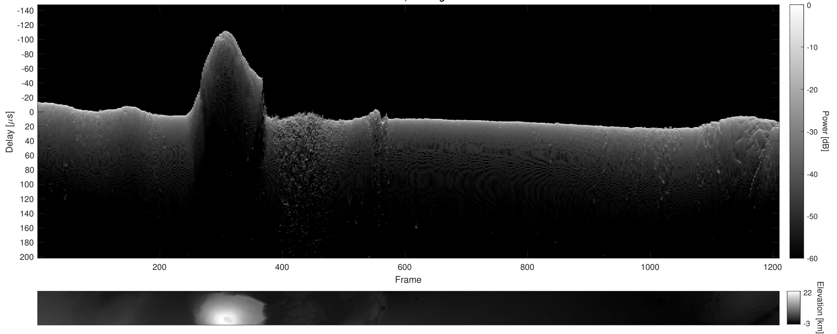
Orbit 10054, Cluttergram
