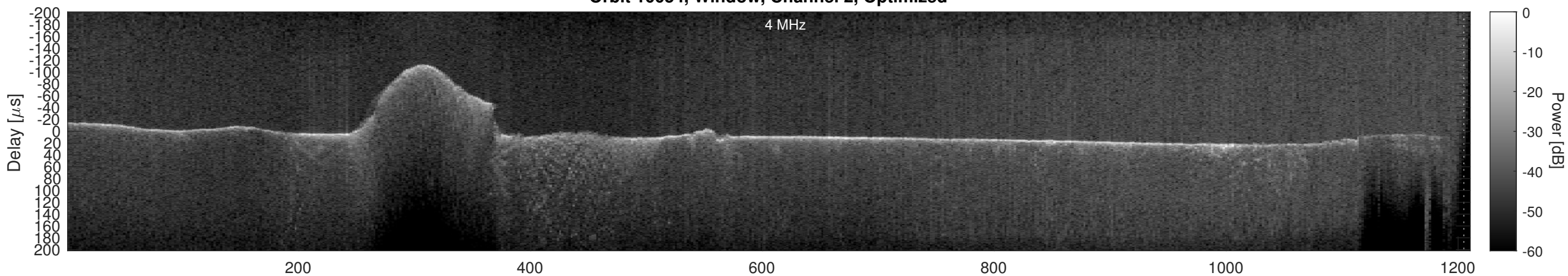
Orbit 10054, Cluttergram
