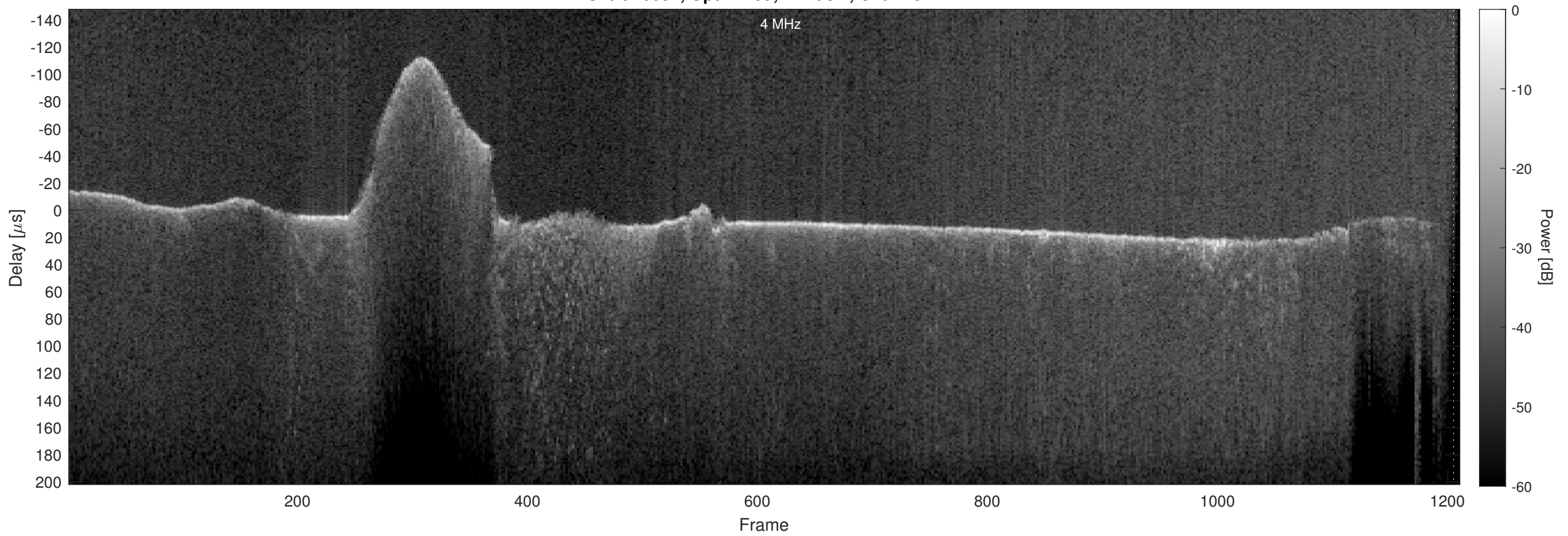
Orbit 10054, Optimized, Window, Channel 2
