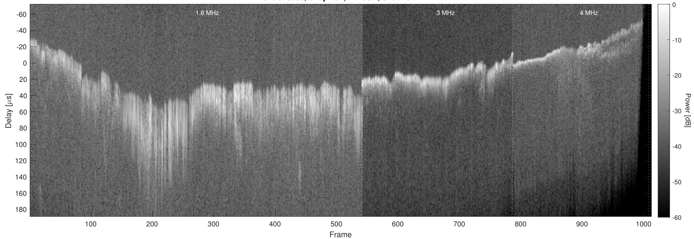
Orbit 10055, Chapman, Window, Channel 2
