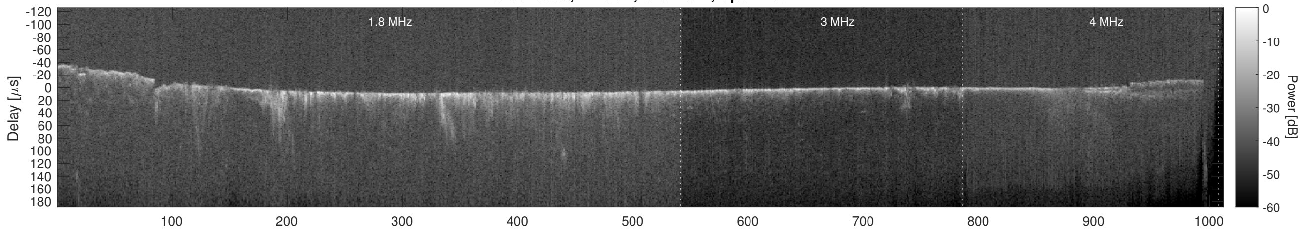
Orbit 10055, Cluttergram
