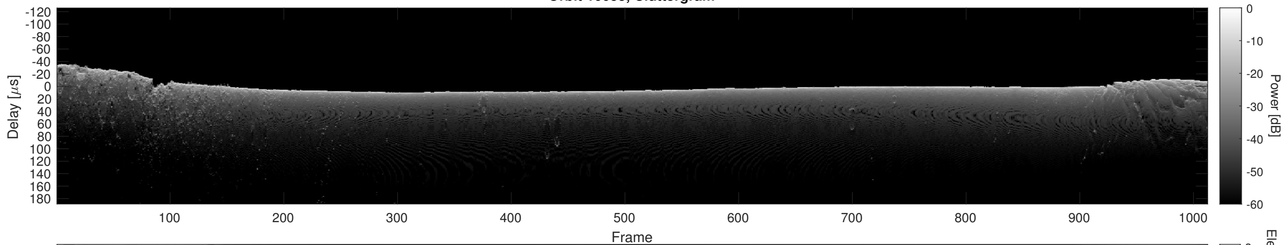
Orbit 10055, Cluttergram
