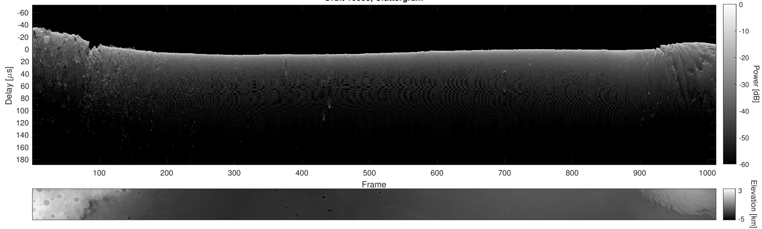
Orbit 10055, Cluttergram
