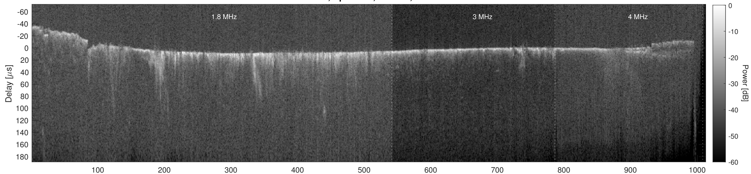
Orbit 10055, Cluttergram
