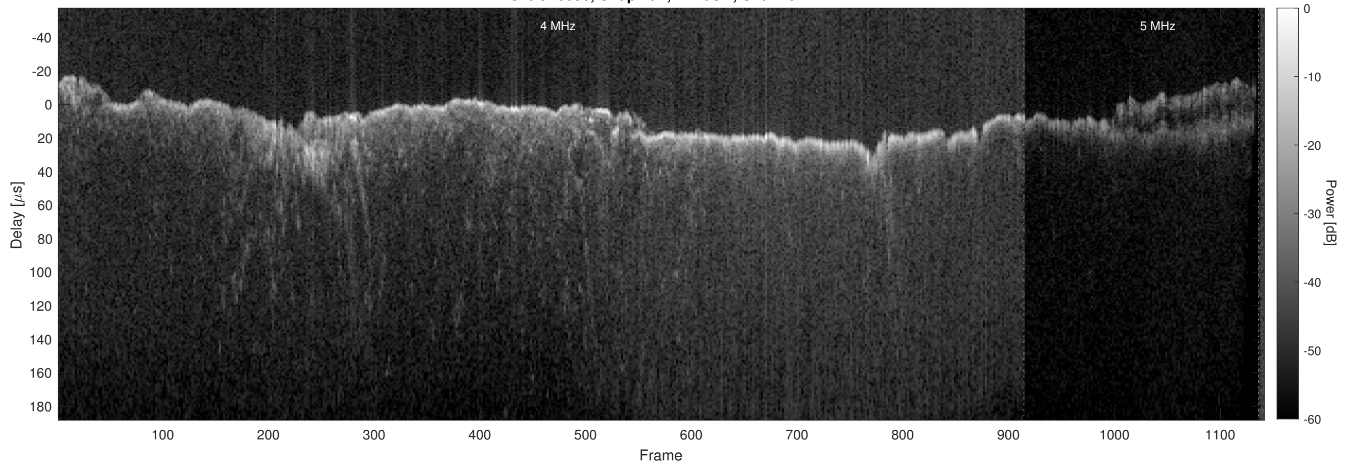
Orbit 10056, Chapman, Window, Channel 2
