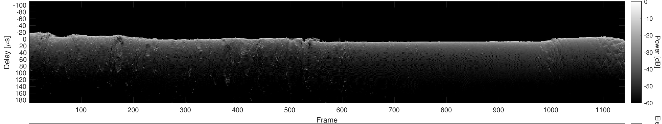
Orbit 10056, Cluttergram
