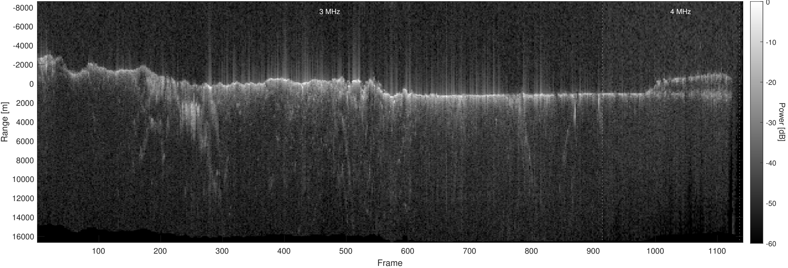
Orbit 10056, Optimized, No Window, Depth-Corrected, Channel 2
