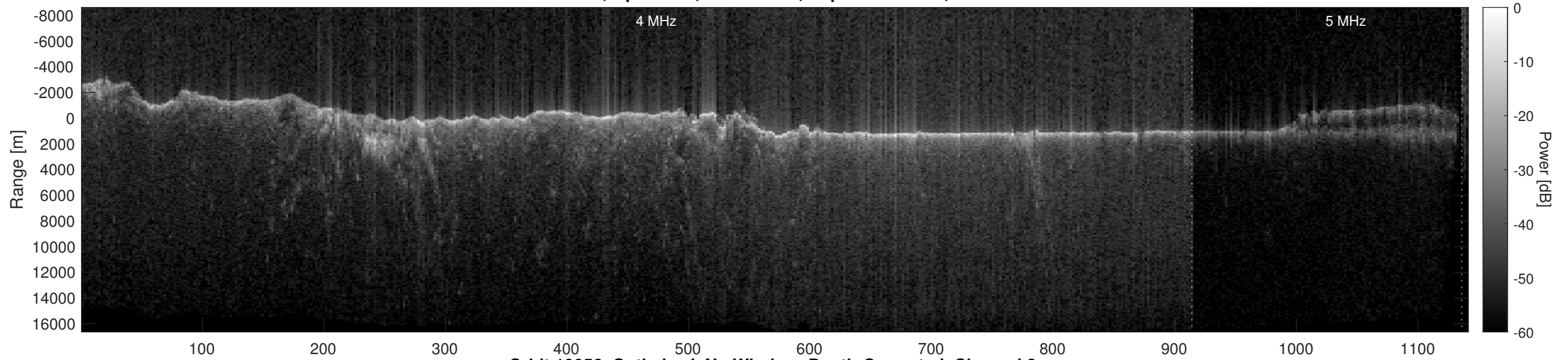
Orbit 10056, Optimized, No Window, Depth-Corrected, Channel 2
