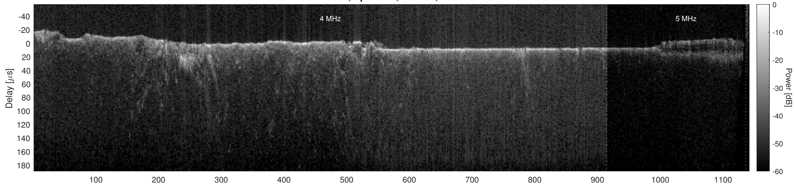
Orbit 10056, Optimized, Window, Channel 2
