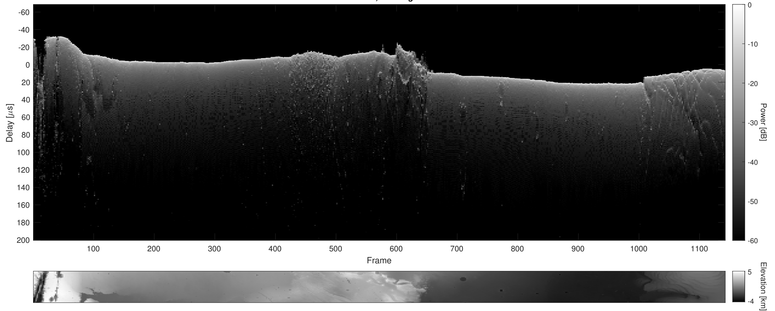
Orbit 10057, Cluttergram
