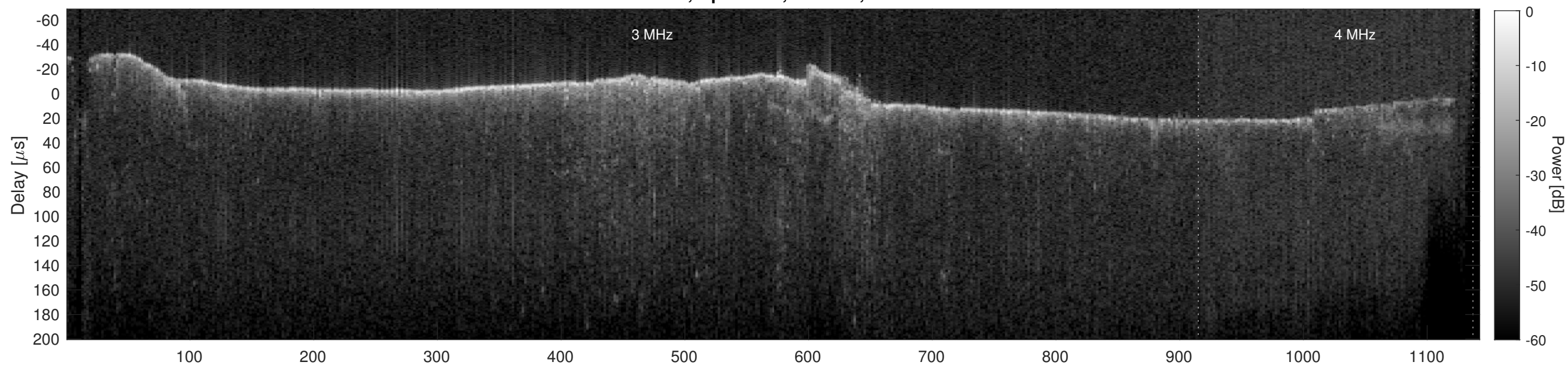
Orbit 10057, Cluttergram
