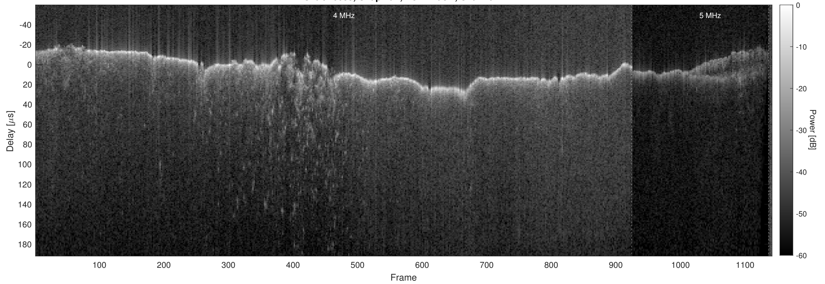
Orbit 10059, Chapman, No Window, Channel 2
