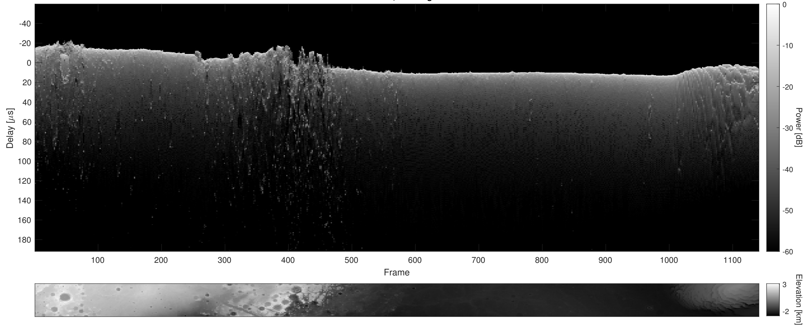
Orbit 10059, Cluttergram
