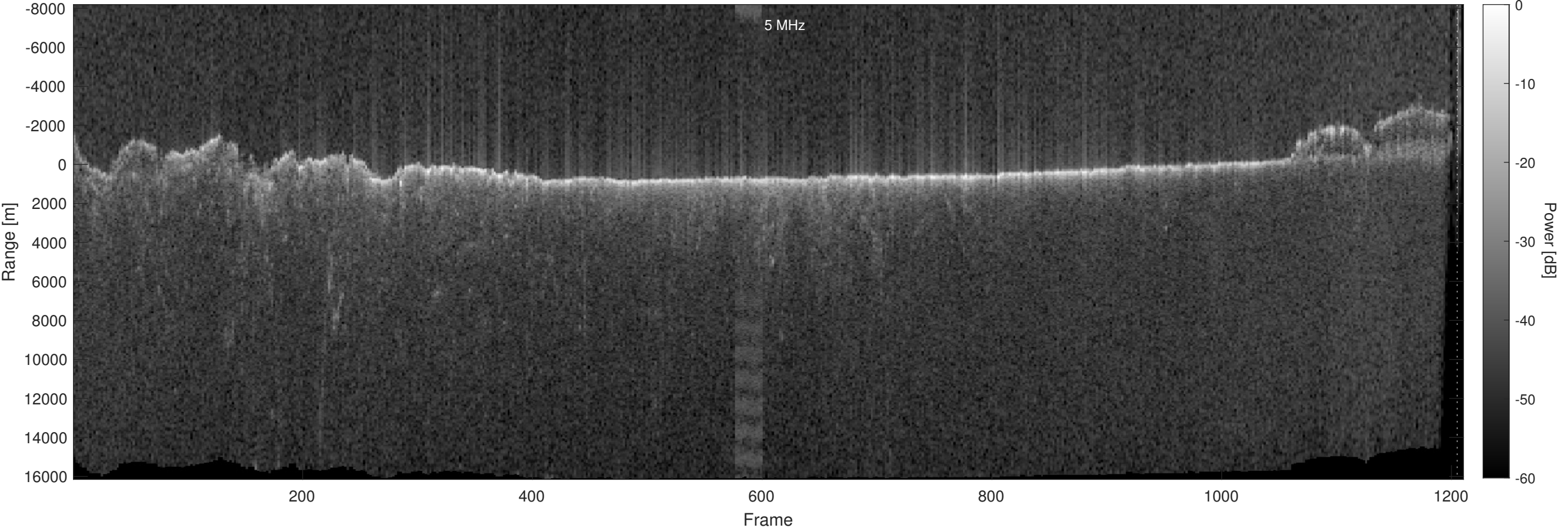
Orbit 10060, Optimized, Window, Depth-Corrected, Channel 2
