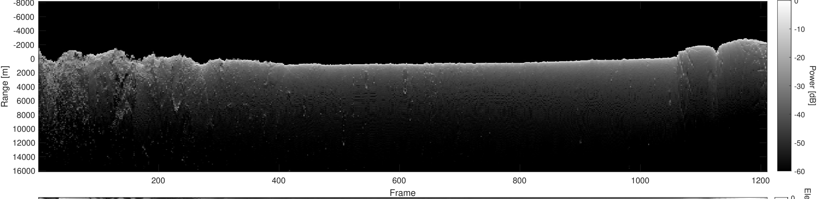
Orbit 10060, Depth-Corrected Cluttergram
