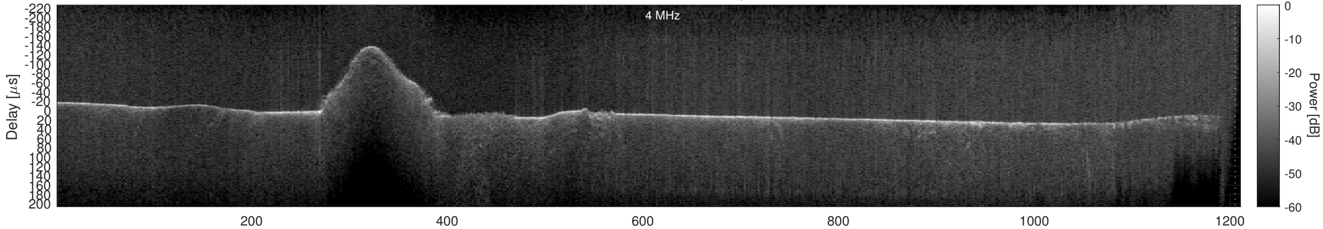
Orbit 10061, Cluttergram
