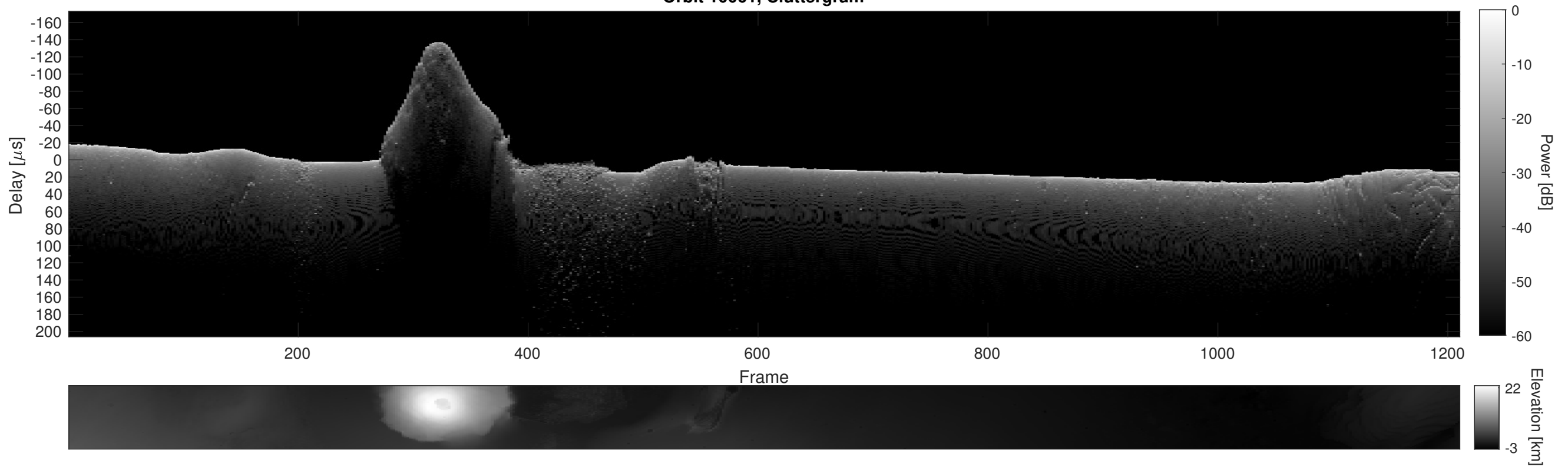
Orbit 10061, Cluttergram
