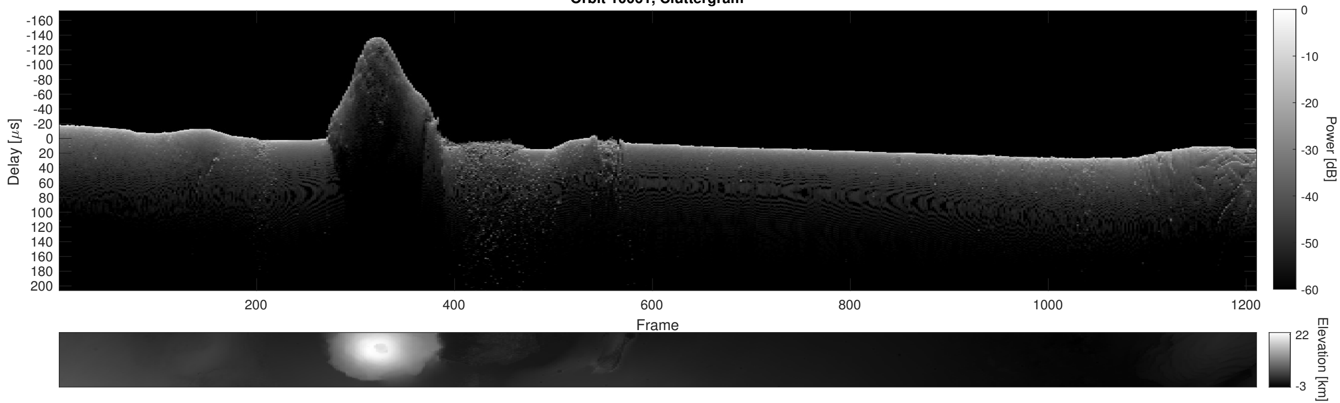
Orbit 10061, Cluttergram
