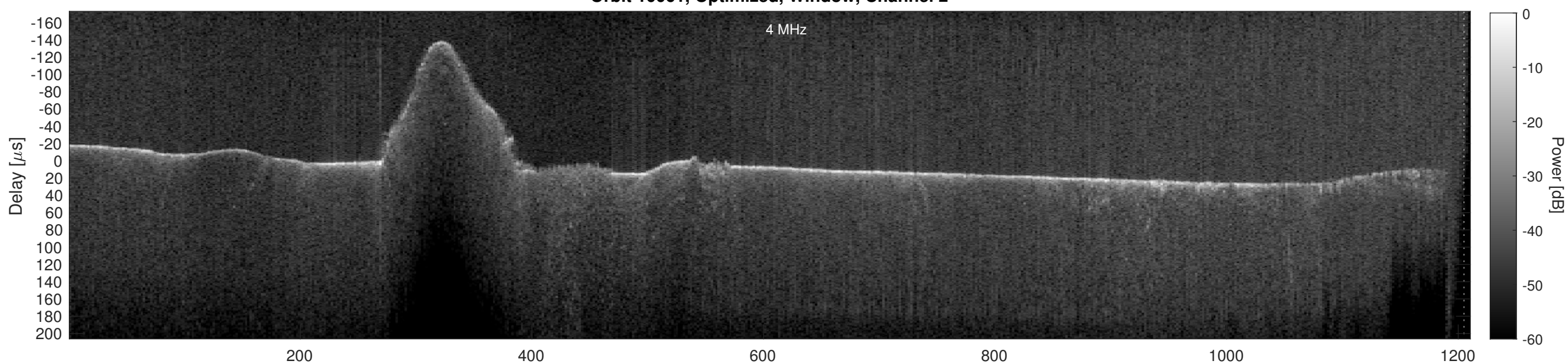
Orbit 10061, Cluttergram
