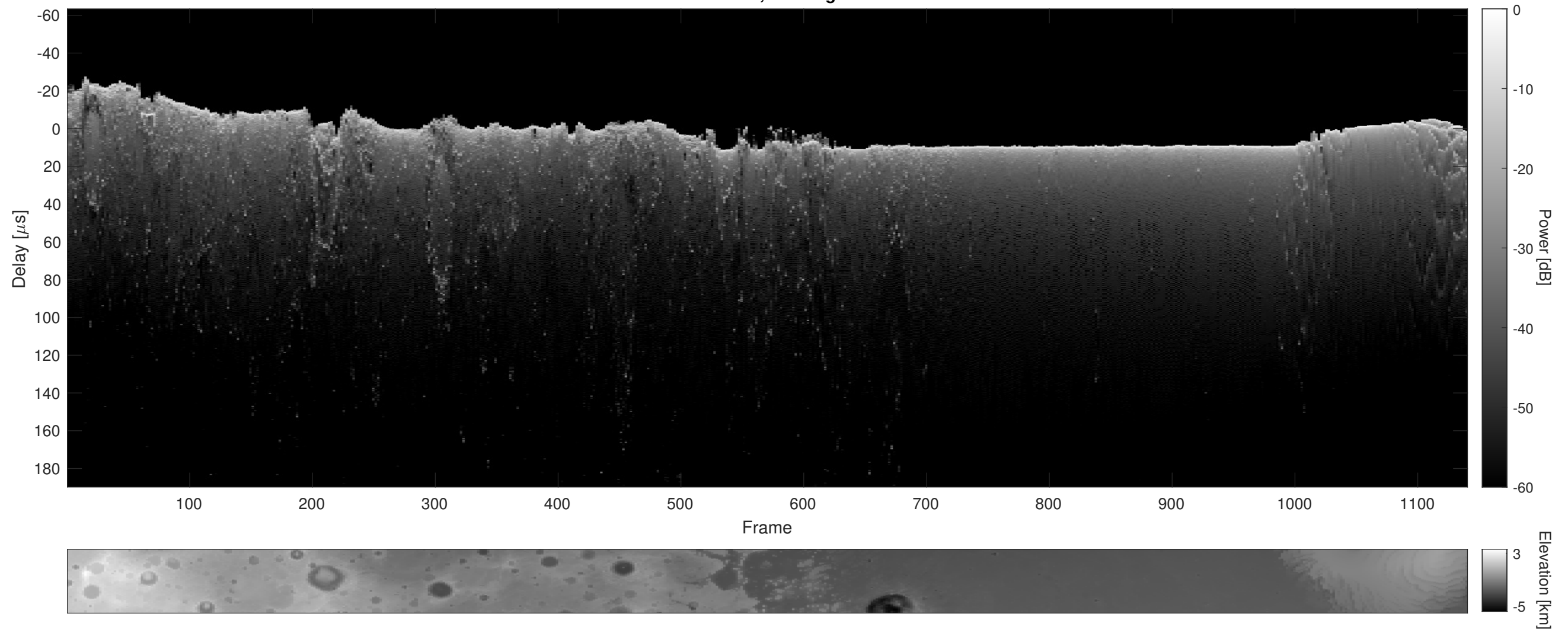
Orbit 10063, Cluttergram
