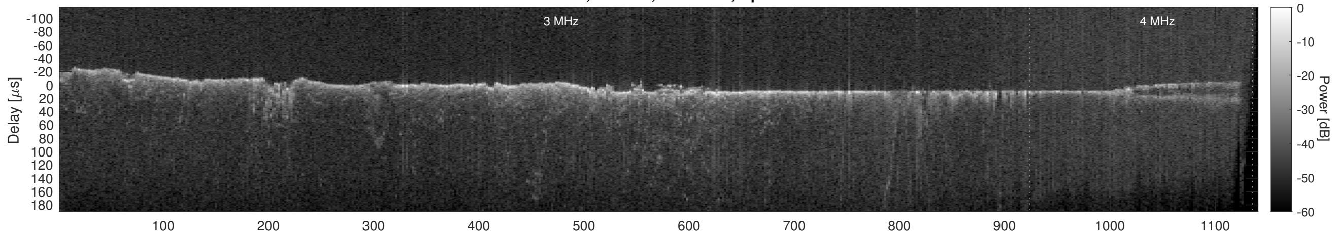
Orbit 10063, Cluttergram
