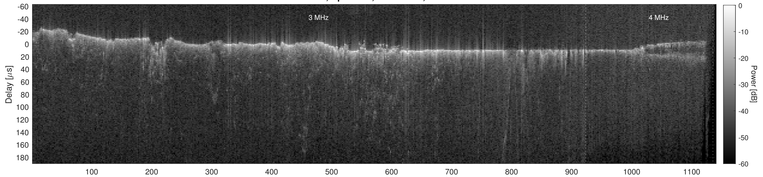
Orbit 10063, Cluttergram
