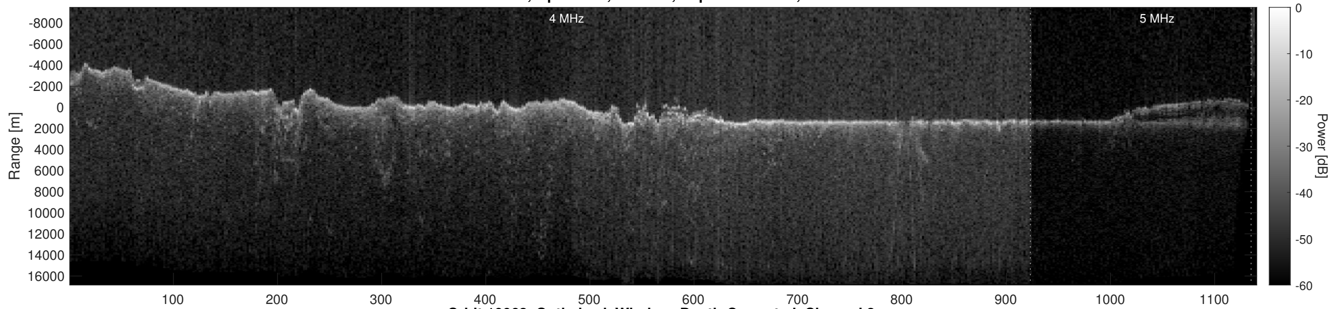
Orbit 10063, Optimized, Window, Depth-Corrected, Channel 2
