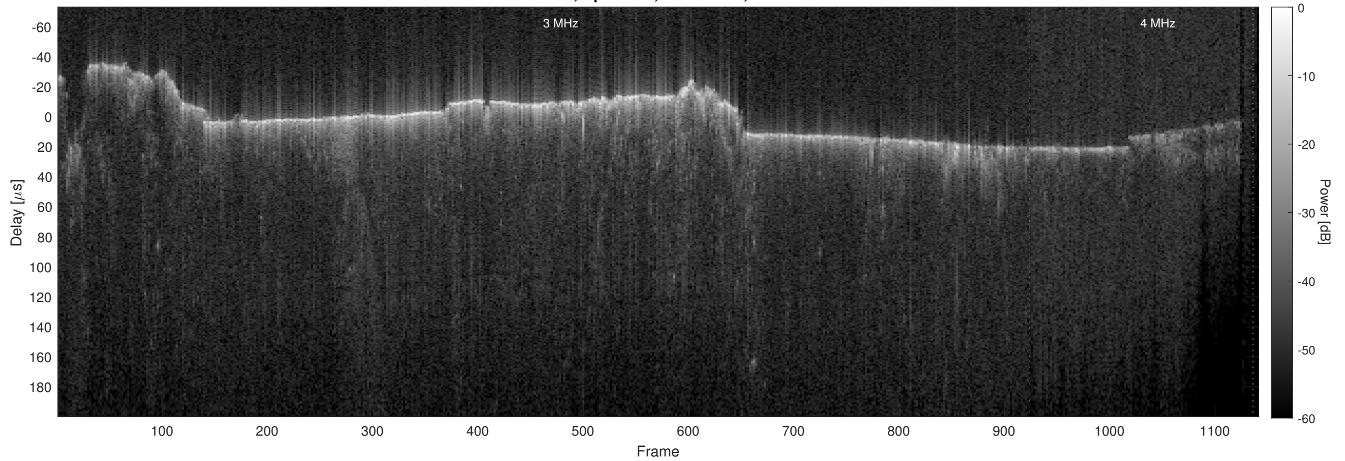
Orbit 10064, Optimized, No Window, Channel 2
