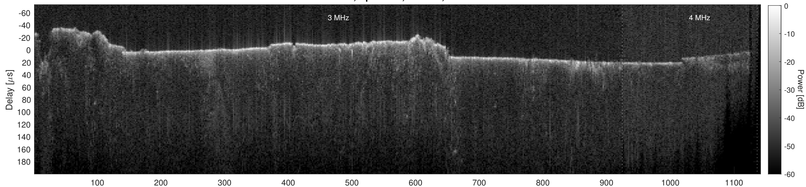
Orbit 10064, Cluttergram
