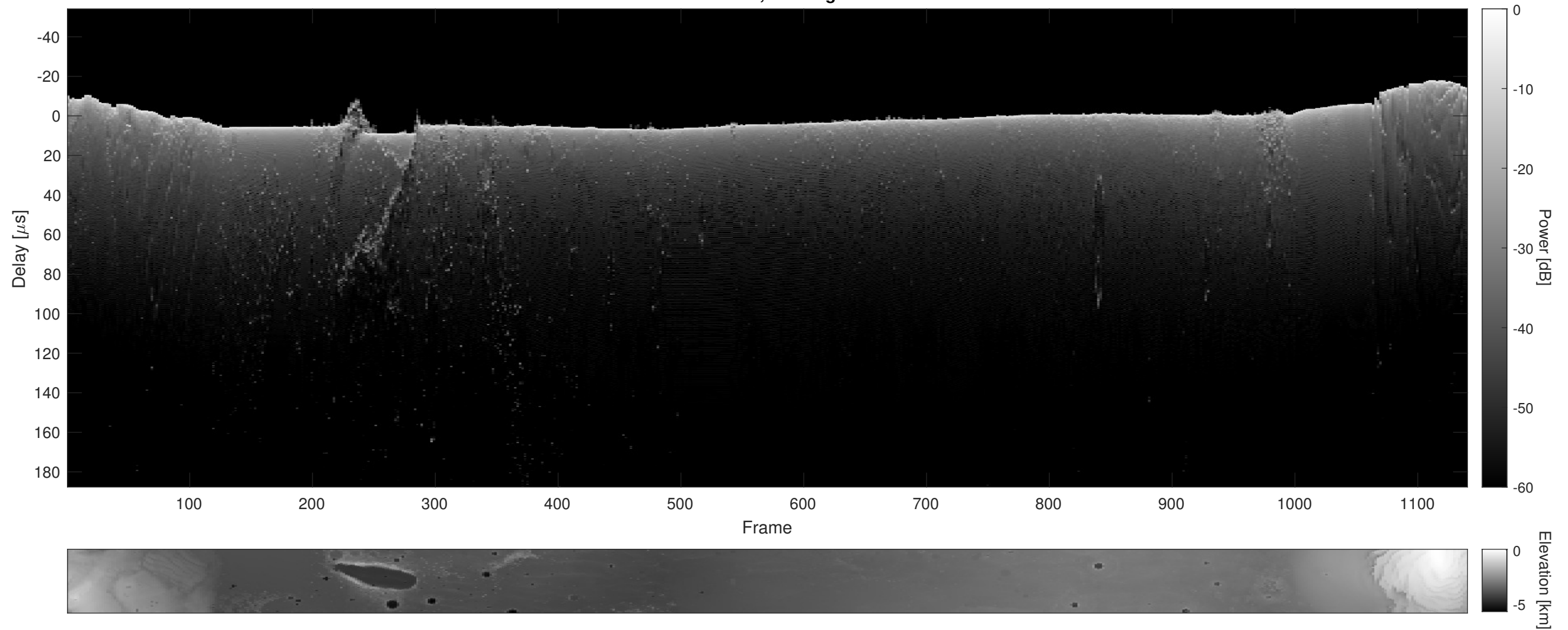
Orbit 10065, Cluttergram
