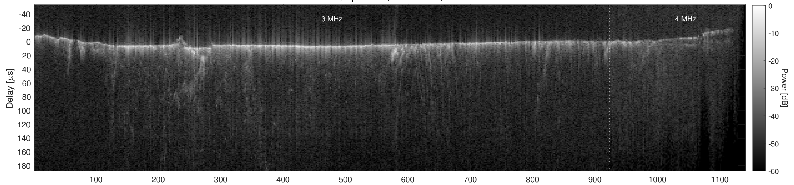
Orbit 10065, Cluttergram
