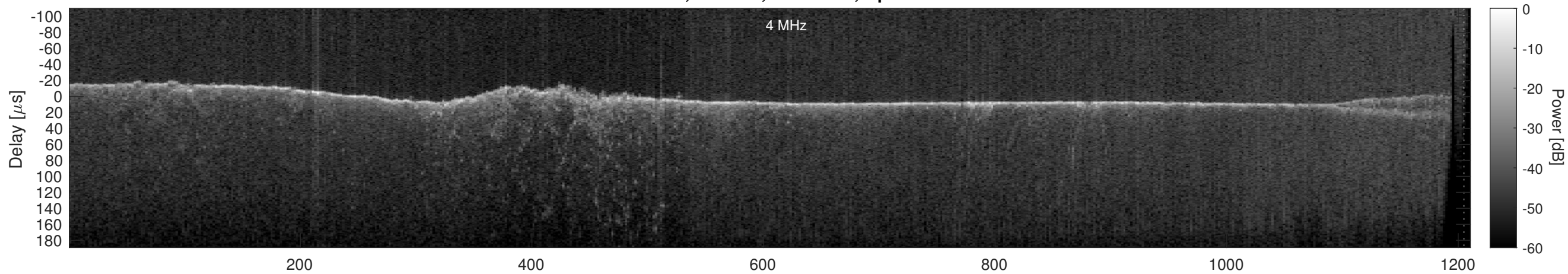
Orbit 10066, Cluttergram
