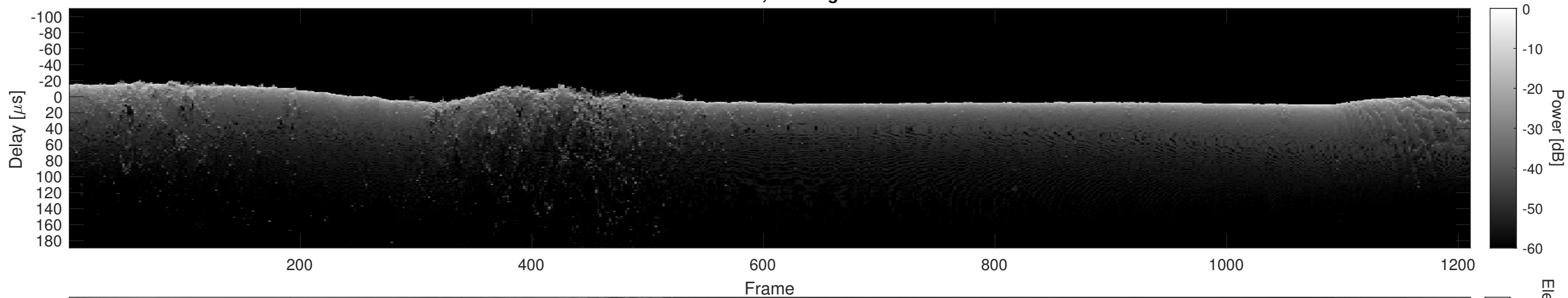
Orbit 10066, Cluttergram
