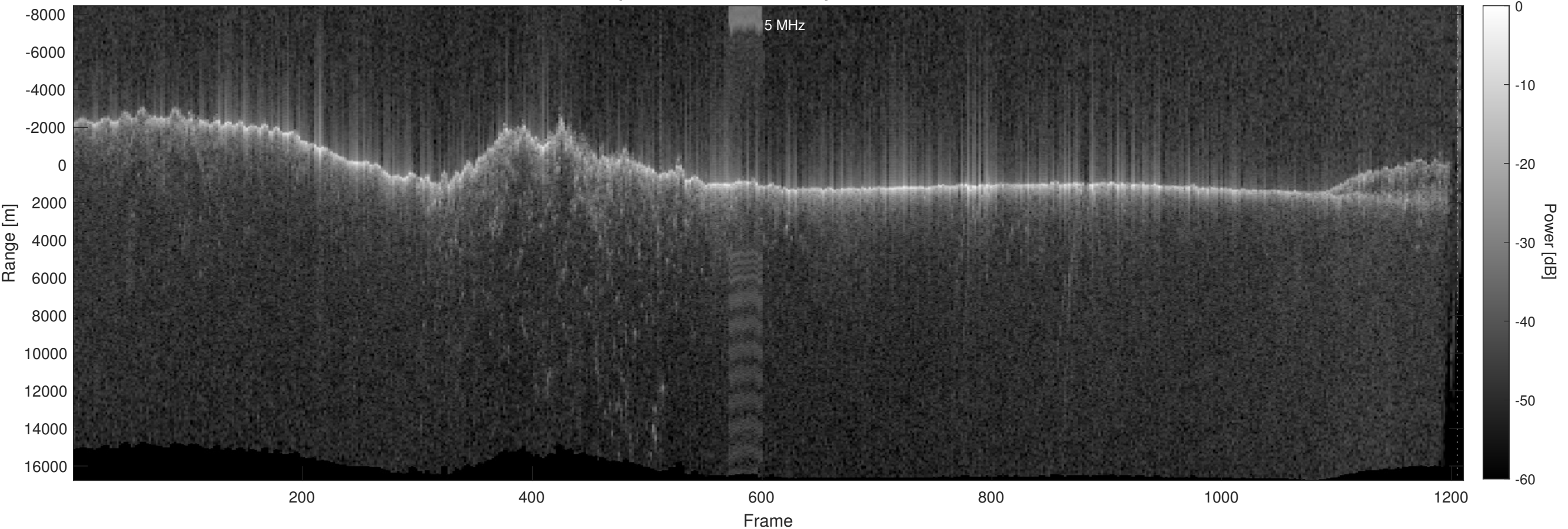
Orbit 10066, Optimized, No Window, Depth-Corrected, Channel 2
