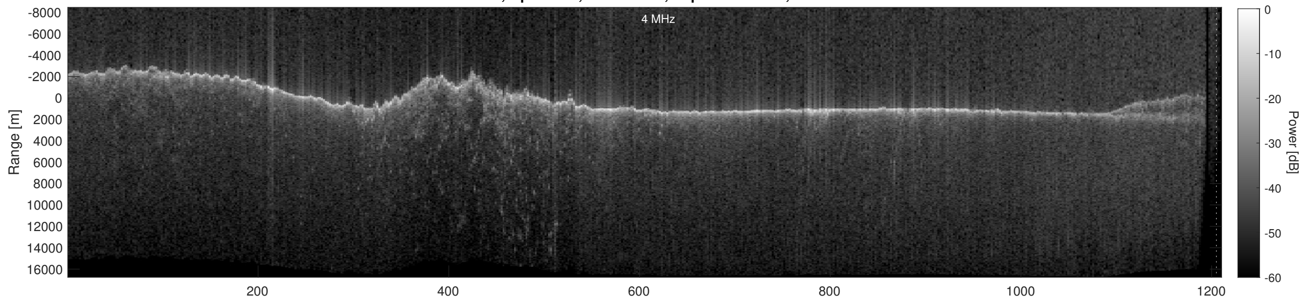
Orbit 10066, Depth-Corrected Cluttergram
