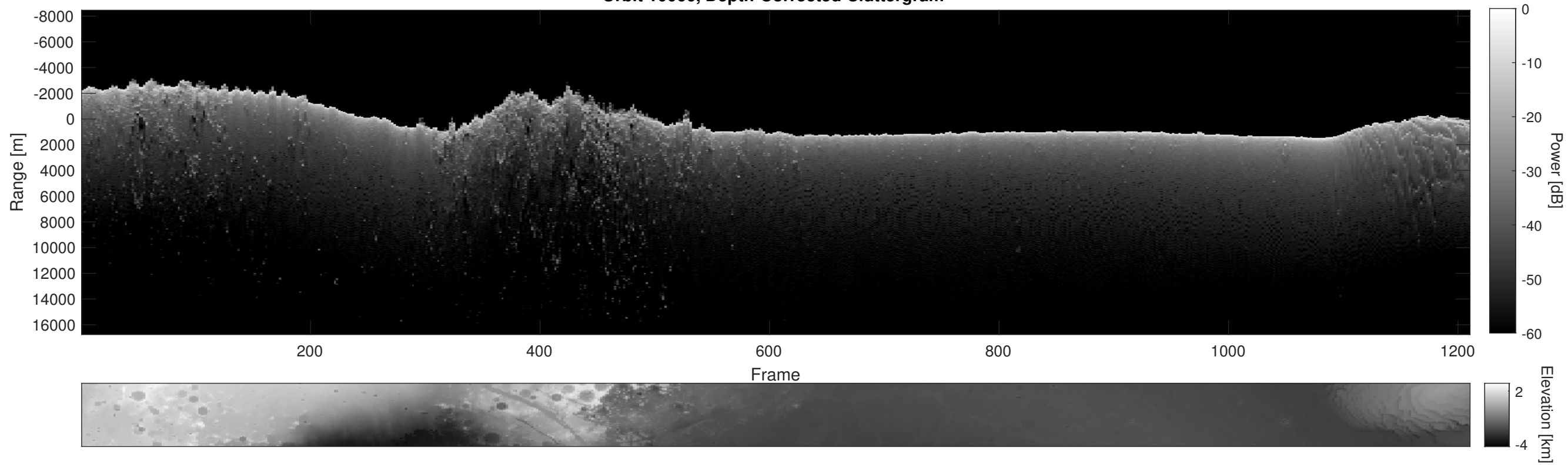
Orbit 10066, Depth-Corrected Cluttergram
