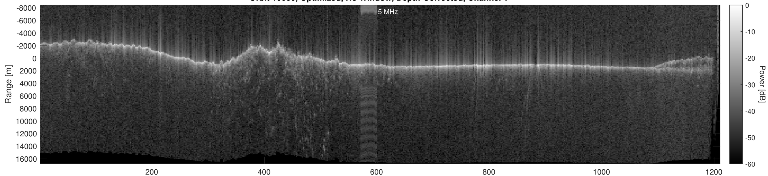
Orbit 10066, Optimized, No Window, Depth-Corrected, Channel 2
