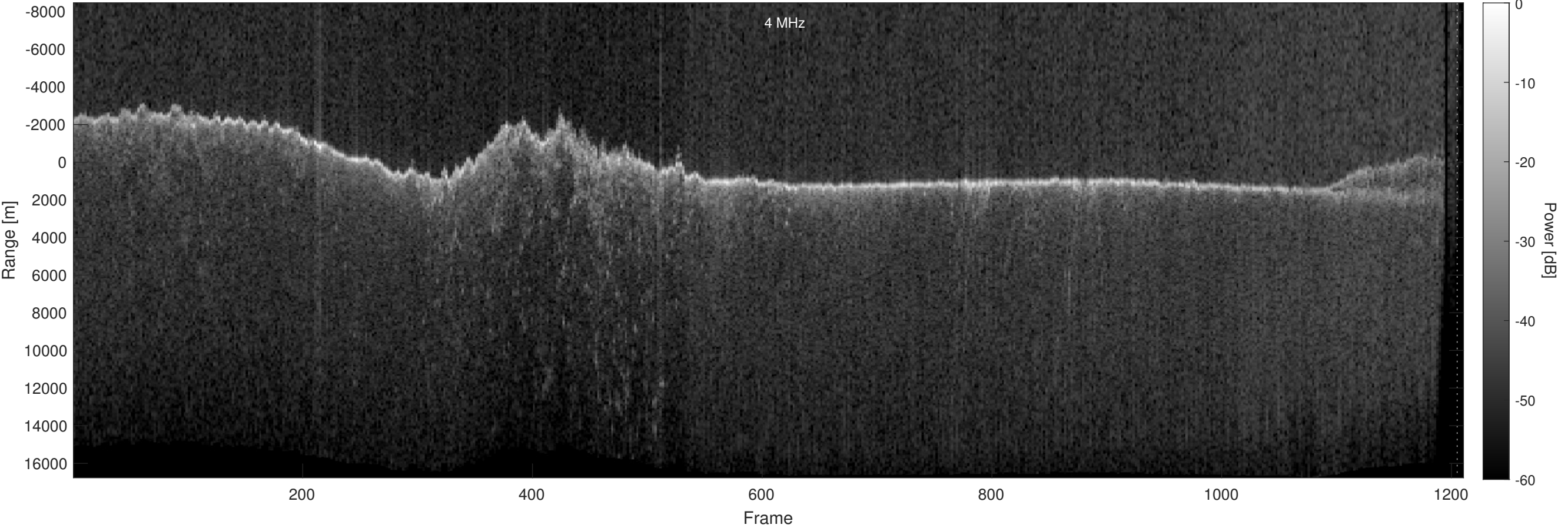
Orbit 10066, Optimized, Window, Depth-Corrected, Channel 2
