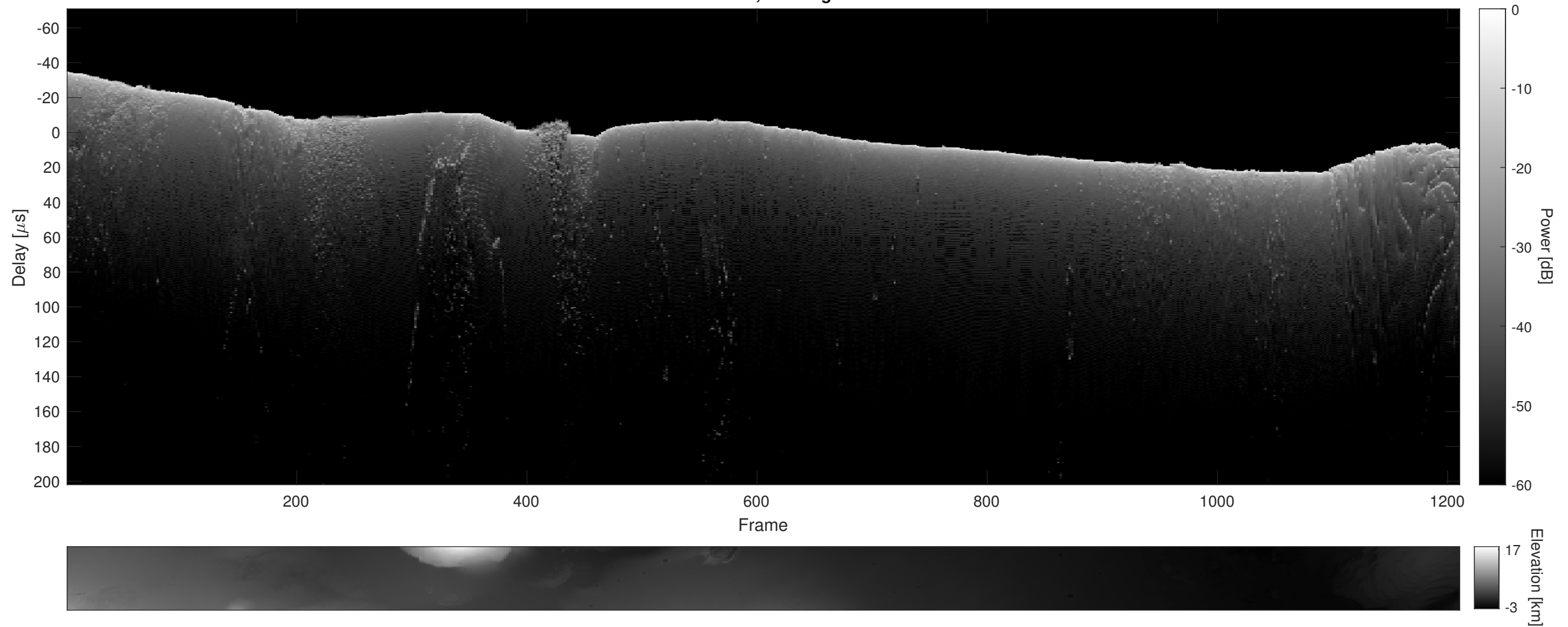
Orbit 10068, Cluttergram
