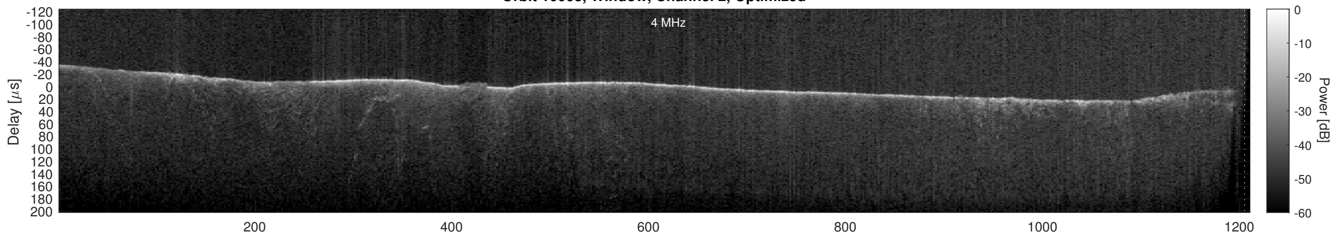
Orbit 10068, Cluttergram
