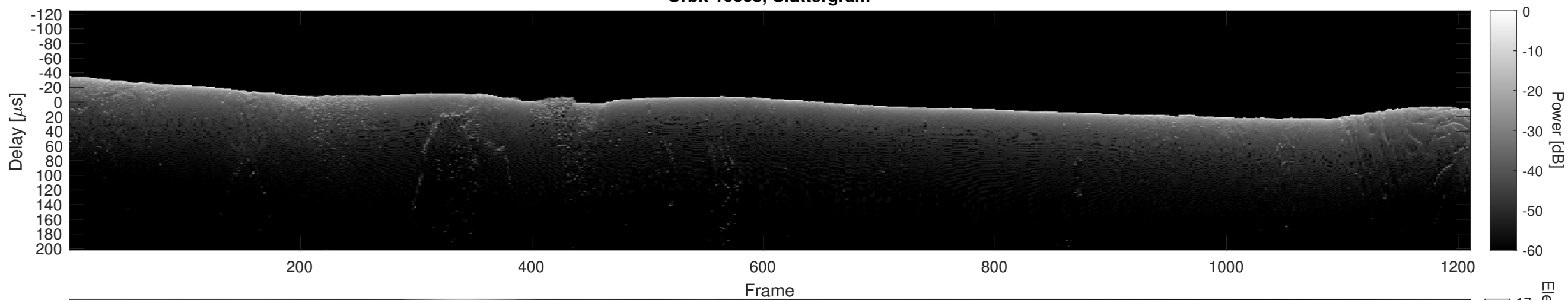
Orbit 10068, Cluttergram
