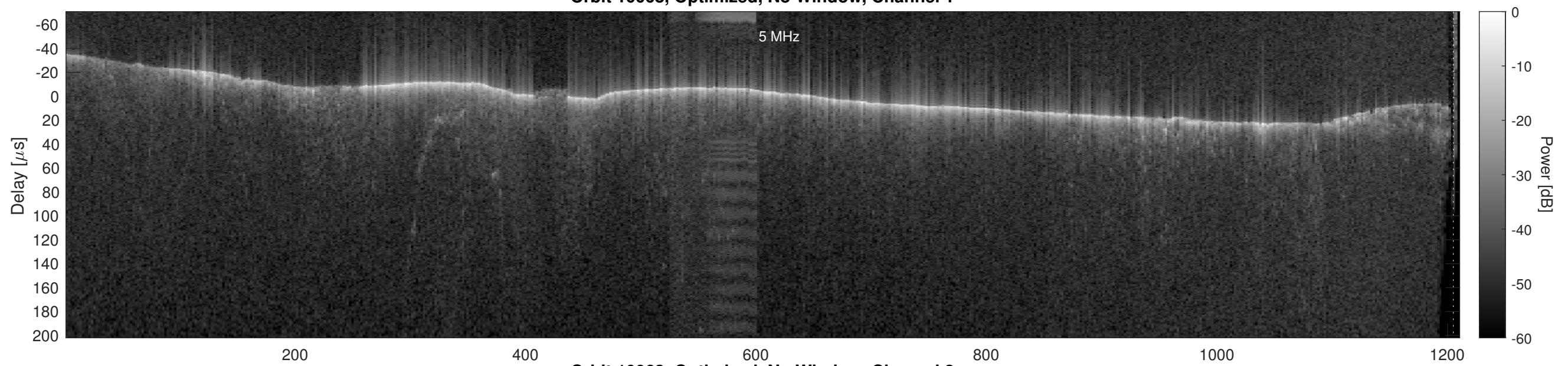
Orbit 10068, Optimized, No Window, Channel 2
